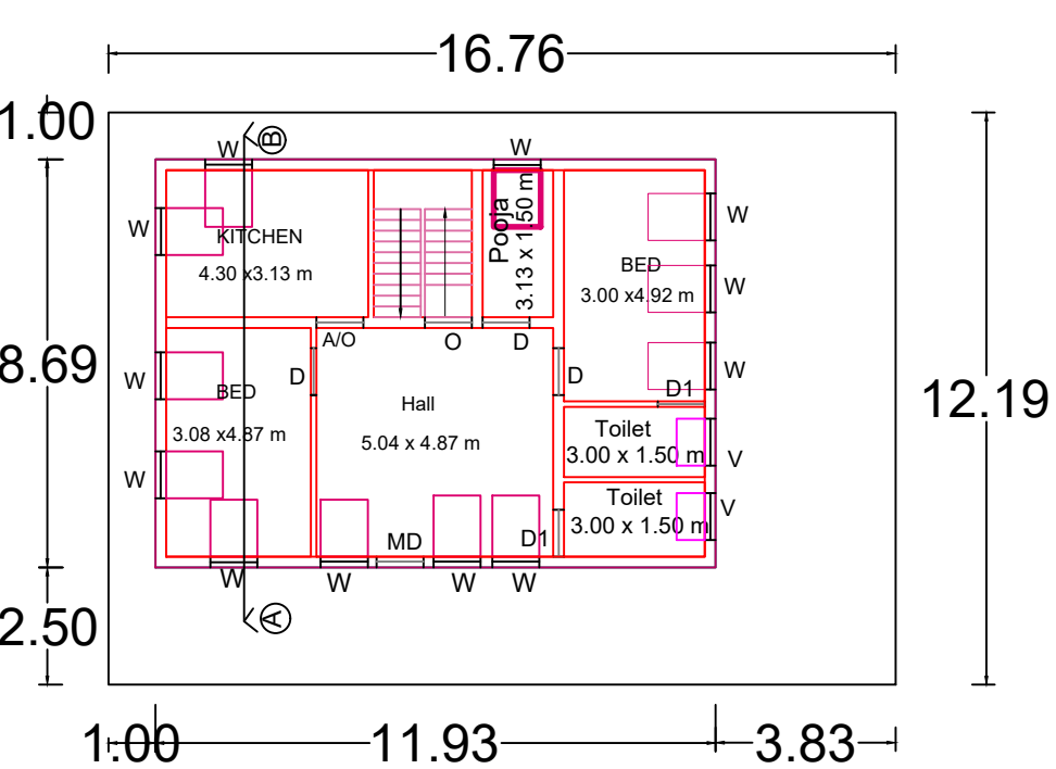
GROUND FLOOR PLAN (North Facing)
