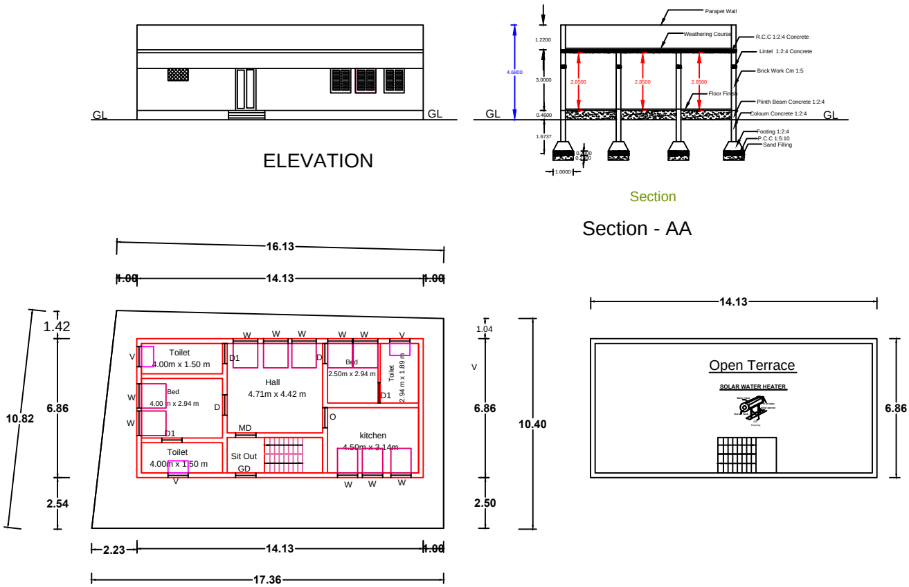
Open Terrace
