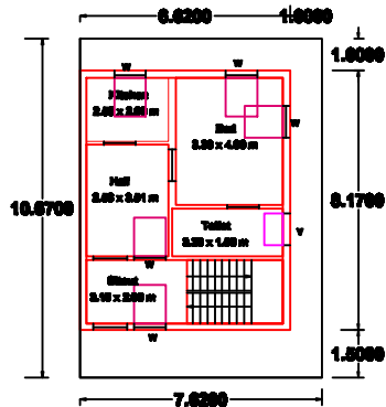
GROUND FLOOR PLAN - EAST FACING
