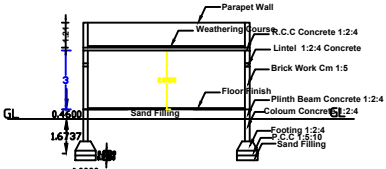
Section Section - AA
