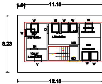
Existing GROUND FLOOR PLAN - WEST & EAST FACING Mr. P.KARUPPASAMY & SEETHALAKSHMI
