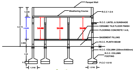
Section SECTION ON 'AA'
