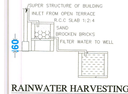
RAINWATER HARVESTING
