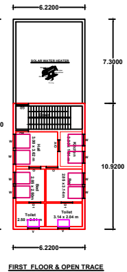
FIRST FLOOR & OPEN TRACE
