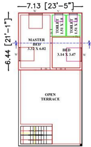
FIRST FLOOR PLAN (EAST FACING)
