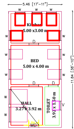
GROUND FLOOR PLAN NORTH FACING
