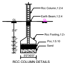
RCC COLUMN DETAILS
