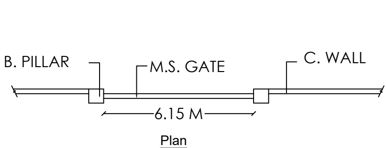
Compound Wall & Gate Details
