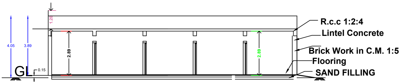
SECTION- AB
