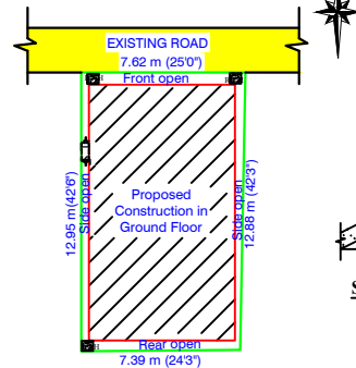
SITE PLAN SCALE 1:200
