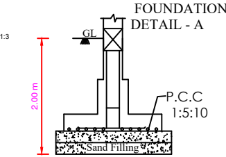
Isolated Footing -A (1.50X1.50)
