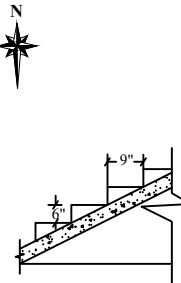
Staircase Detail Not To Scale
