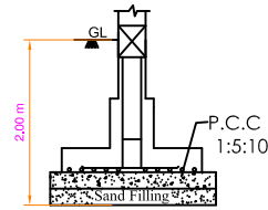
Isolated Footing - A (1.50X1.50) (Not to Scale)
