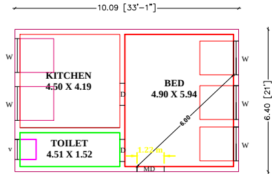
GROUND FLOOR PLAN {EAST FACING}
