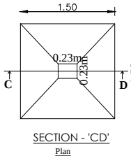
Using 'U' type trap 2 Nos in inlet, outlet & Ventpipe will be covered with mosquito proof covering net in inner side of vent pipe and top of vent pipe. Septic Tank With U Trap Not To Scale
