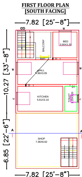
FIRST FLOOR PLAN [SOUTH FACING]
