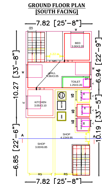
GROUND FLOOR PLAN [SOUTH FACING]
