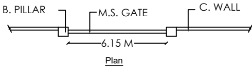
Compound Wall & Gate Details
