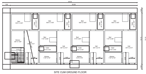
SITE CUM GROUND FLOOR
