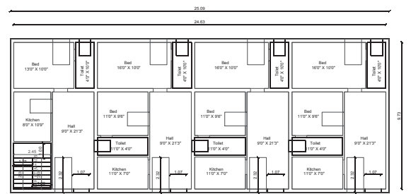
SITE CUM FIRST FLOOR
