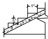
Staircase Detail Not To Scale
