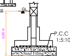
Isolated Footing - A (1.50X1.50) (Not to Scale)
