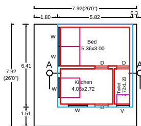
PLAN - G.F ( Facing North )
