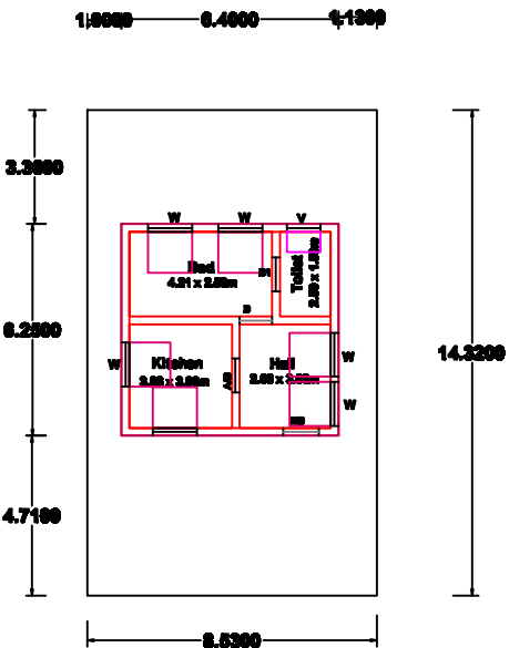
GROUND FLOOR PLAN ( EAST FACING )
