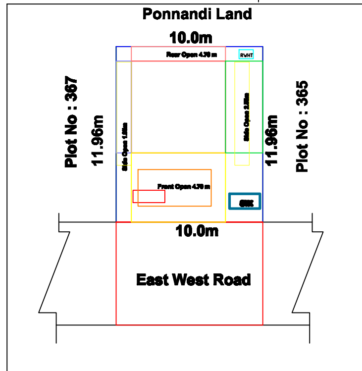
Site Plan
