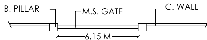
Compound Wall & Gate Details
