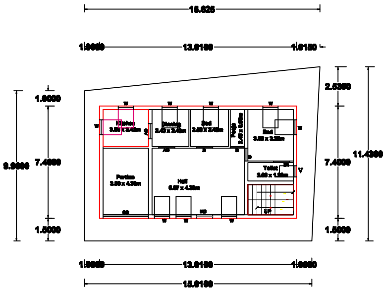
EXISTING GROUND FLOOR PLAN ( NORTH FACING )
