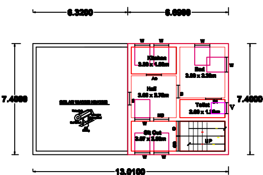
PROPOSED FIRST FLOOR PLAN & OPEN TERRACE EAST FACING )
