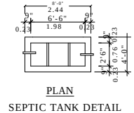
SEPTIC TANK DETAIL
