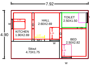
GROUND FLOOR PLAN (Facing East)
