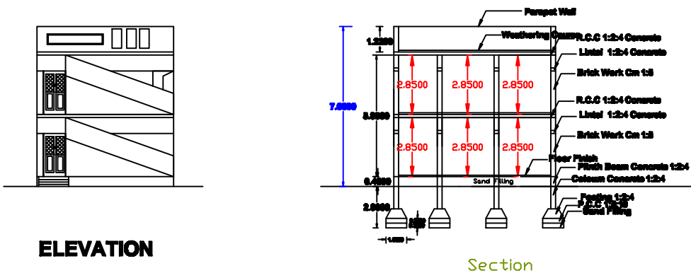
Section
