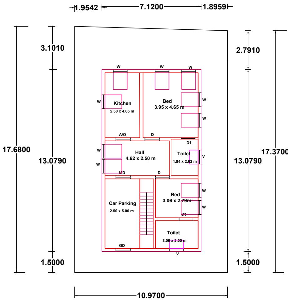
GROUND FLOOR North Facing
