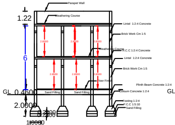
Section Section - AA
