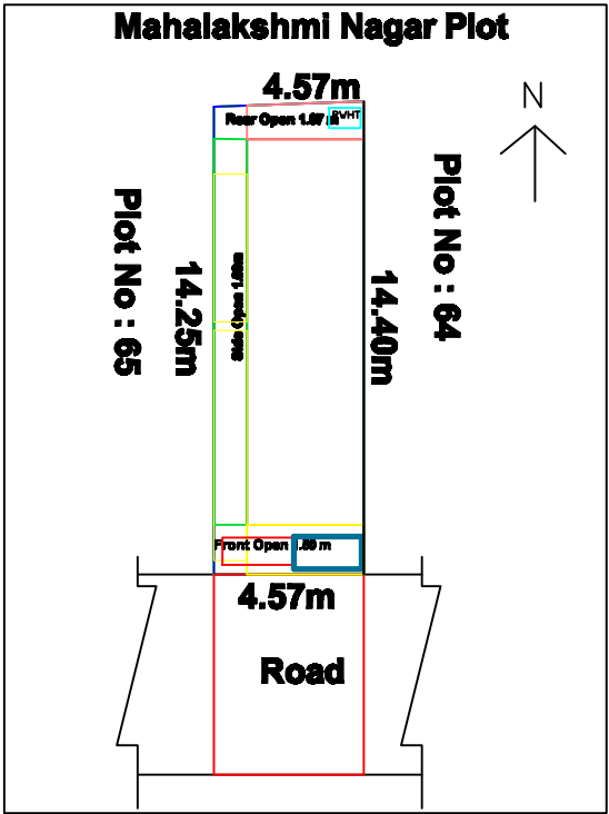
Site Plan
