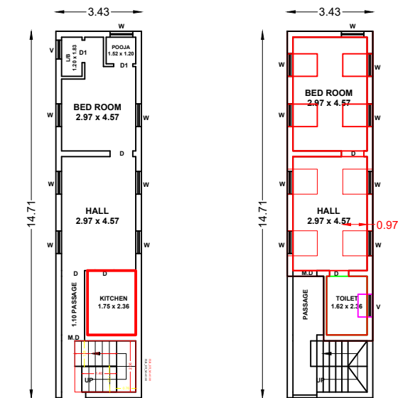
EXISTING GROUND FLOOR PLAN (SOUTH FACING)
