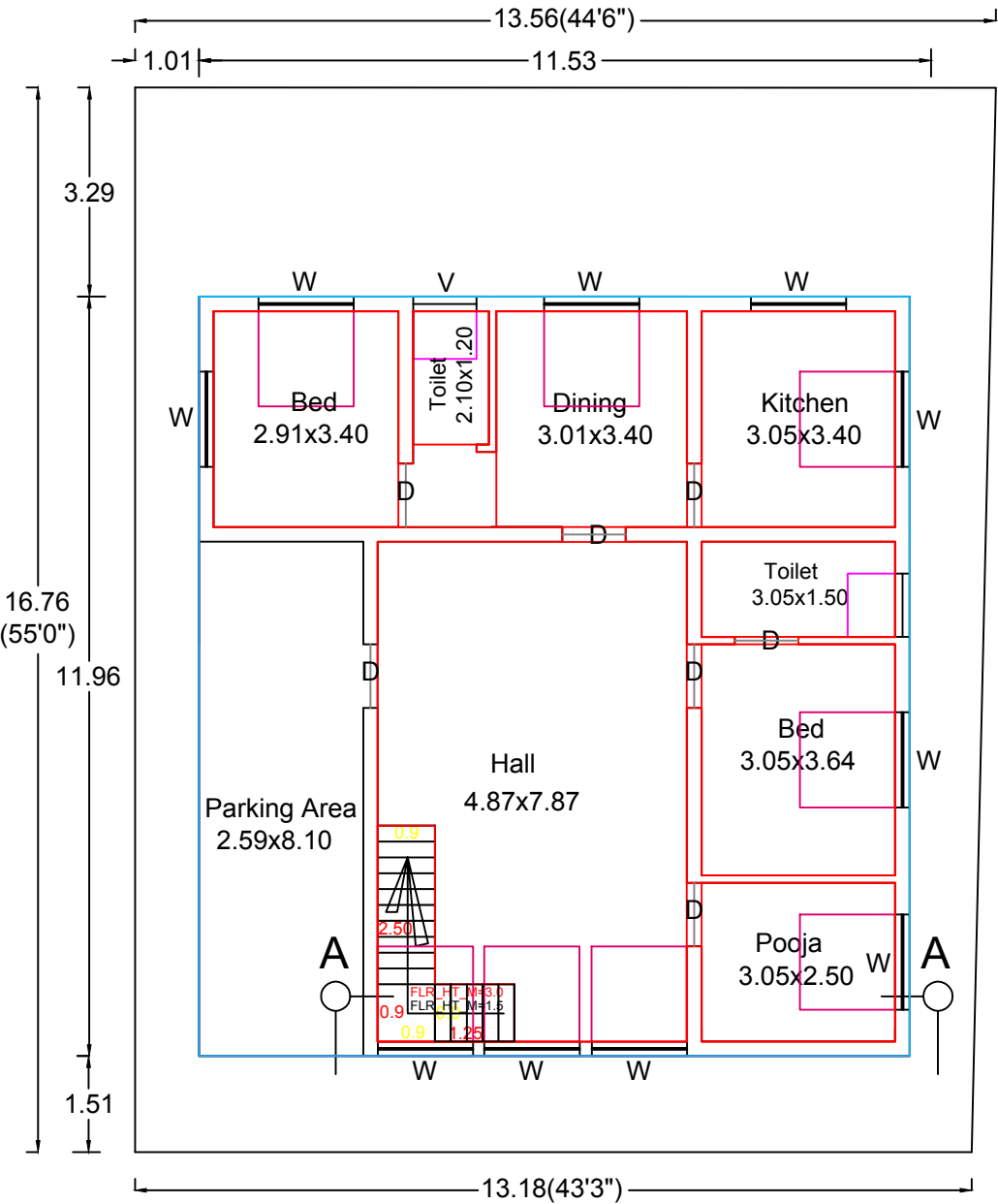
PLAN - G.F ( Facing WEST)
