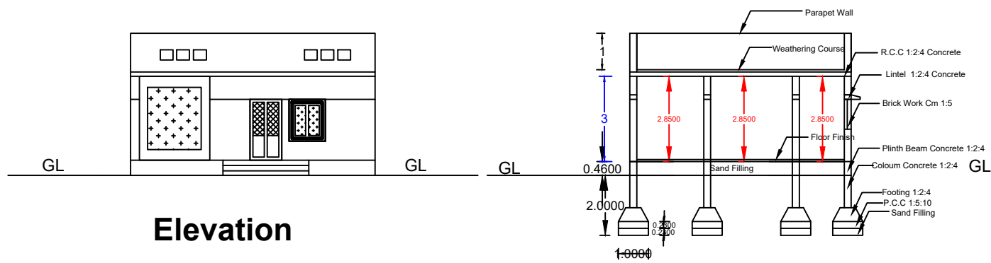
Section - AA
