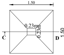
SECTION - 'CD' FOUNDATION DETAIL - A
