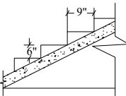
Staircase Detail Not To Scale
