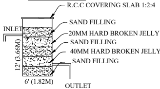
Waste Water Recyle Unit Not To Scale
