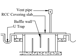
Waste Water Recyle Unit Not To Scale
