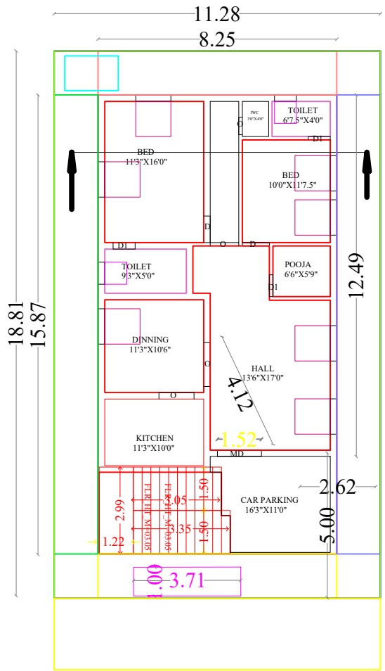
GROUND FLOOR PLAN (FACEING OF EAST)
