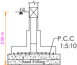
Isolated Footing -A (1.50X1.50) (Not to Scale)
