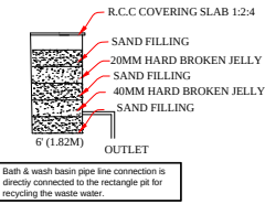
Waste Water Recycle Unit Not To Scale
