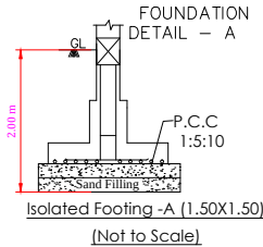
Isolated Footing -A (1.50X1.50) (Not to Scale)
