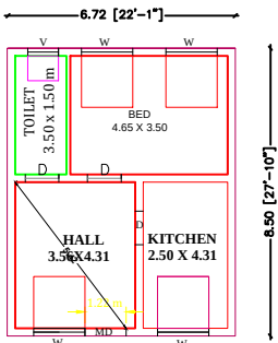
GROUND FLOOR PLAN ( SOUTH FACING )
