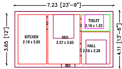
EX GROUND FLOOR PLAN [EAST FACING]
