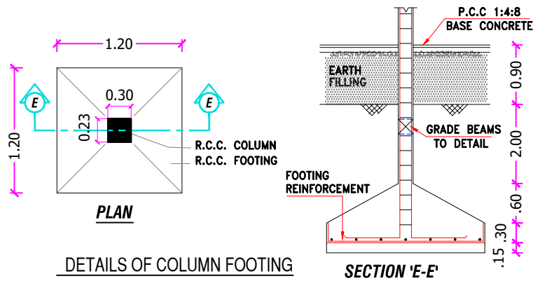
DETAILS OF COLUMN FOOTING
