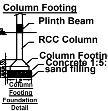
Column Footing
