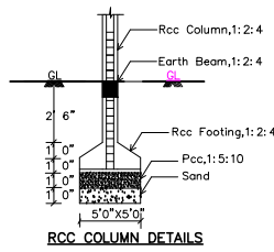
RCC COLUMN DETAILS
