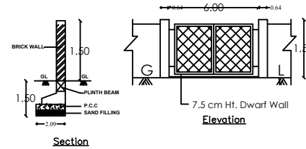
Section
