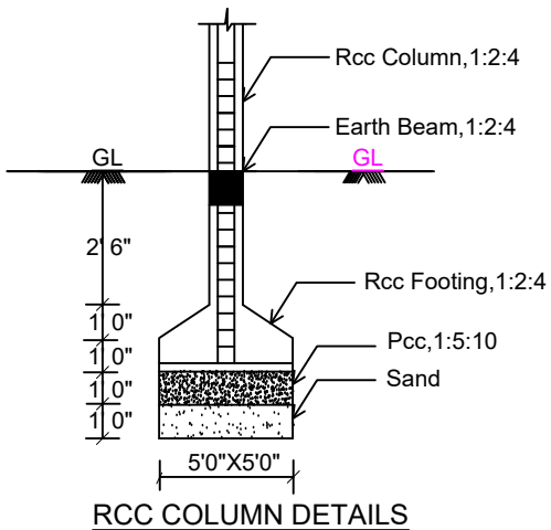
RCC COLUMN DETAILS
