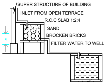
RAINWATER HARVESTING
