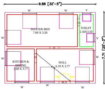
GROUND FLOOR PLAN (EAST FACING)
