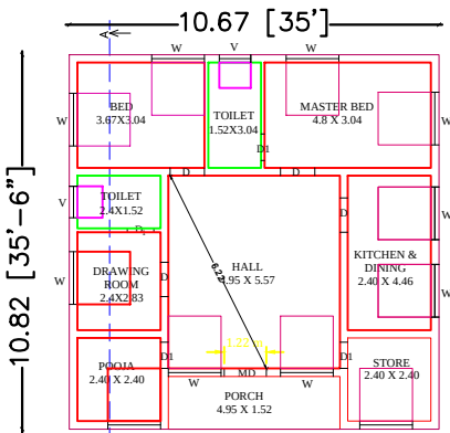
GROUND FLOOR PLAN (SOUTH FACING)
