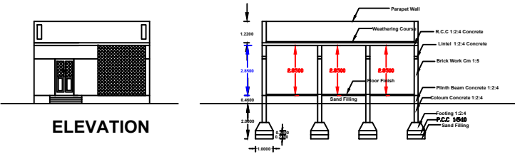
Section Section - AA
