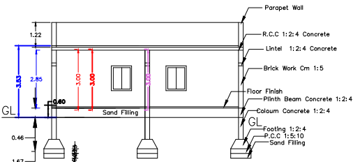
Section Section - AA
