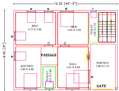
GROUND FLOOR PLAN NORTH FACING
