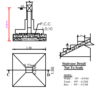
Isolated Footing - A (1.50X1.50) (Not to Scale)
