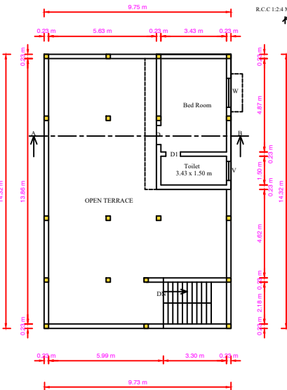
PROPOSED SECOND FLOOR PLAN
