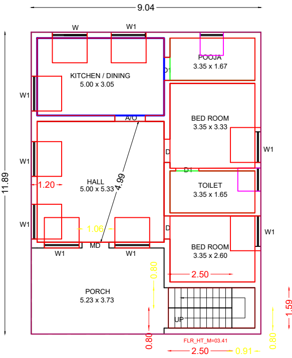
GROUND FLOOR (NORTH FACING)
