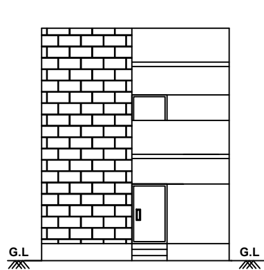
FRONT ELEVATION
