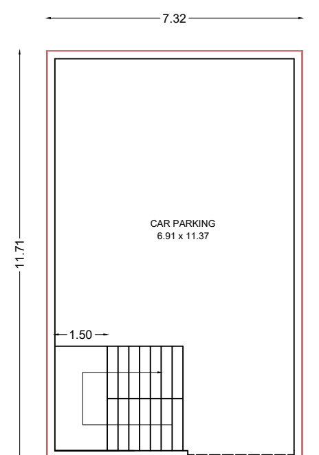
GROUND FLOOR PLAN (WEST FACING)
