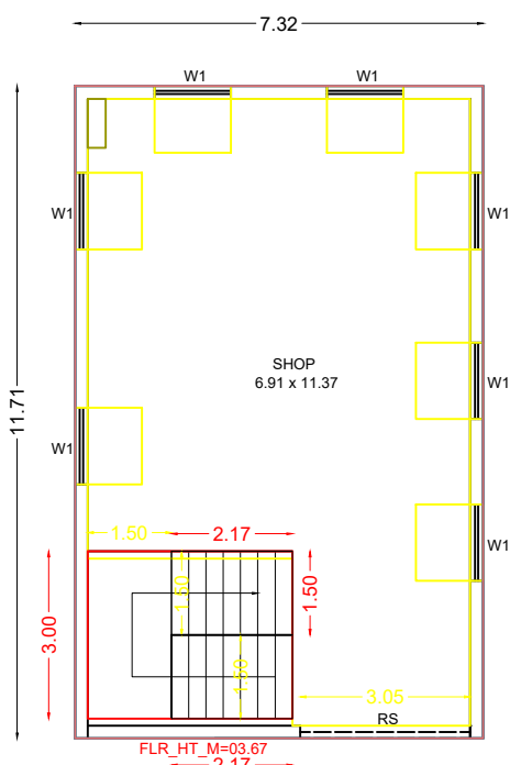
GROUND FLOOR PLAN (WEST FACING)
