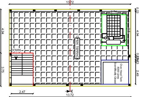
FLOOR - TERRACE
