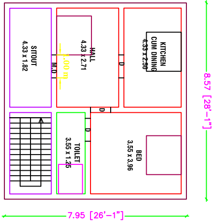
GROUND FLOOR PLAN [NORTH FACING]
