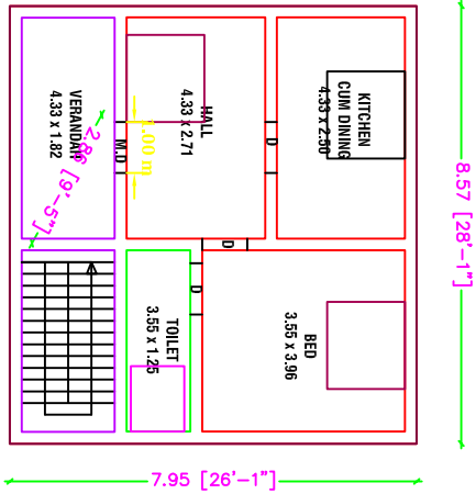
FIRST FLOOR PLAN [NORTH FACING]
